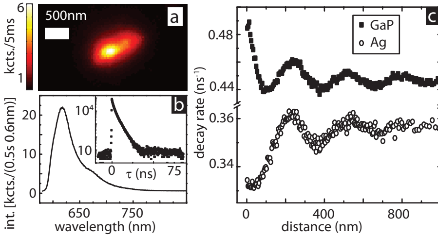
Figure 7.5: (a) Confocal fluorescence-intensity image of a superemitter manufactured from a GaP NW of nominally 100 nm in diameter and 1 \mu m in length. (b) Fluorescence spectrum of superemitter shown in (a), resembling the spectrum of the used dye. Inset shows fluorescence decay trace of superemitter in (a), exhibiting a slightly non-single-exponential decay. (c) Black squares: Decay rate as a function of distance to scanning micro-mirror of superemitter fabricated from GaP nanowire characterized in (a) and (b). Open circles: Decay rate as function of distance to scanning mirror of superemitter fabricated from an Ag nanowire.
