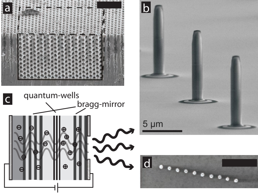
Figure 1.2: (a) 3D photonic-bandgap crystal fabricated in silicon by drilling two perpendicularly oriented arrays of holes into a wafer. Scalebar denotes 4 μm (fabricated by the Complex Photonic Systems group at the University of Twente in collaboration with groups in Dutch industry (ASML, TNO, Philips), see References [27, 28]). (b) Micropillar cavities confining an optical mode in three dimensions by Bragg mirrors in the vertical direction and the pillar-shape in the radial direction (image courtesy of Monika Emmerling, Adriana Wolf, and Prof. Stephan Reitzenstein, Department of Applied Physics at the University of Würzburg. See References [29, 30]). (c) Schematic of VCSEL. The structure consists of epitaxially grown multi-layers sandwiched between Ohmic contacts. Two oppositely doped Bragg mirrors confine the lasing mode to the region of the quantum wells, where carriers are confined and effectively recombine (adopted from Reference [25]). (d) SEM micrograph of silver nanoparticles arranged in a chain. These plasmonic nanoparticles strongly scatter light and can be used to confine propagating radiation (scalebar denotes 500 nm, image courtesy of René de Waele, see Reference [31]).
