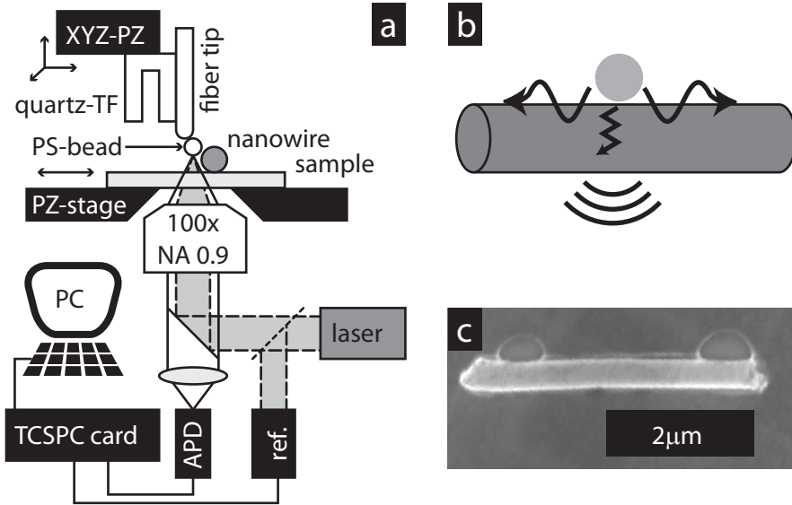
Figure 3.1: (a) Schematic of experimental setup. The fluorescent source is attached to a scanning probe and positioned with respect to the structure of interest. A pulsed pump laser is focused onto the source whose fluorescence is collected by the same microscope objective. The fluorescence is split off by a dichroic beam-splitter and a color filter (not sketched) and focused onto an APD. (b) Schematic of nanowire with light source in its vicinity. The decay channels, radiative, non-radiative, and into surface plasmons are indicated. Plasmons may decay via absorption in the wire or radiation from wire end. (c) SEM micrograph of an Au nanowire.
