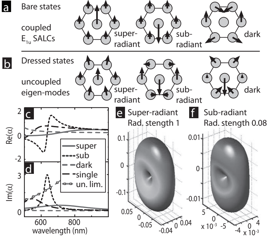
Figure 5.3: (a) Bare-state nondiagonal polarization basis, consisting of a super-radiant, sub-radiant and dark symmetry-adapted linear combination (SALC) of E_{1u} derived from group theory. (b) Dressed-state basis of decoupled super-radiant, sub-radiant and dark eigen-modes (small out-of-phase components not visualized). (c) Real and (d) imaginary parts of polarizabilities of the eigen-modes and a single constituent particle in 10^{-31} \text{Cm}^2/\text{V} . For comparison, in (d) we also plot the unitary limit. (e) and (f) are radiation patterns of super-radiant and sub-radiant eigen-modes in W/sr. Radiative strength indicates total radiated power relative to super-radiant eigen-mode.
